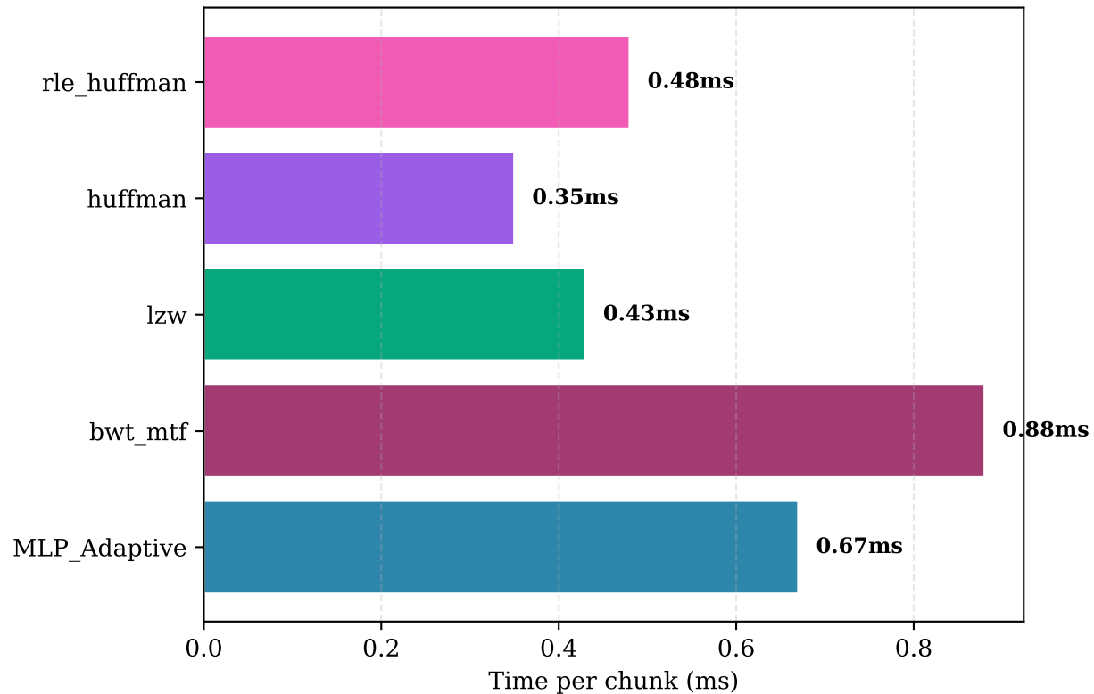
Compression Speed (24% faster)
